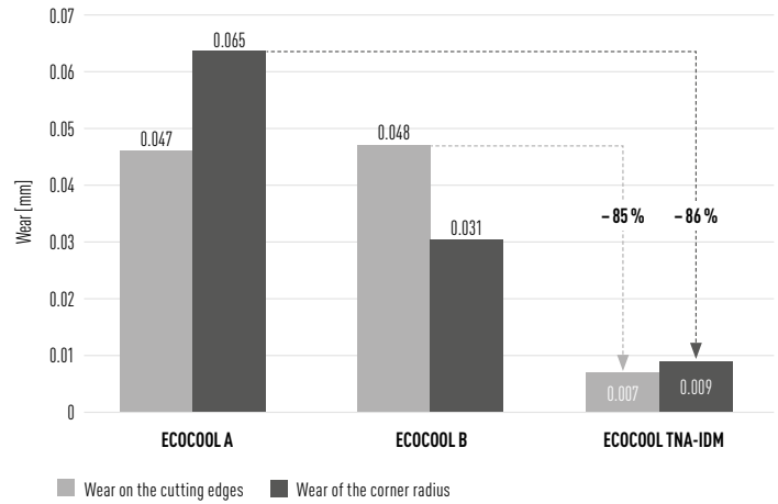
85% less tool wear thanks to ECOCOOOL TNA-IDM.
