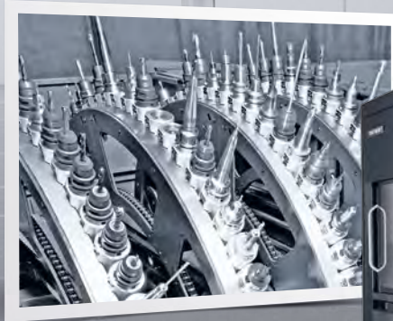
Outer wheel with 63 available tool pockets, inner wheels with 60 available tool pockets.
