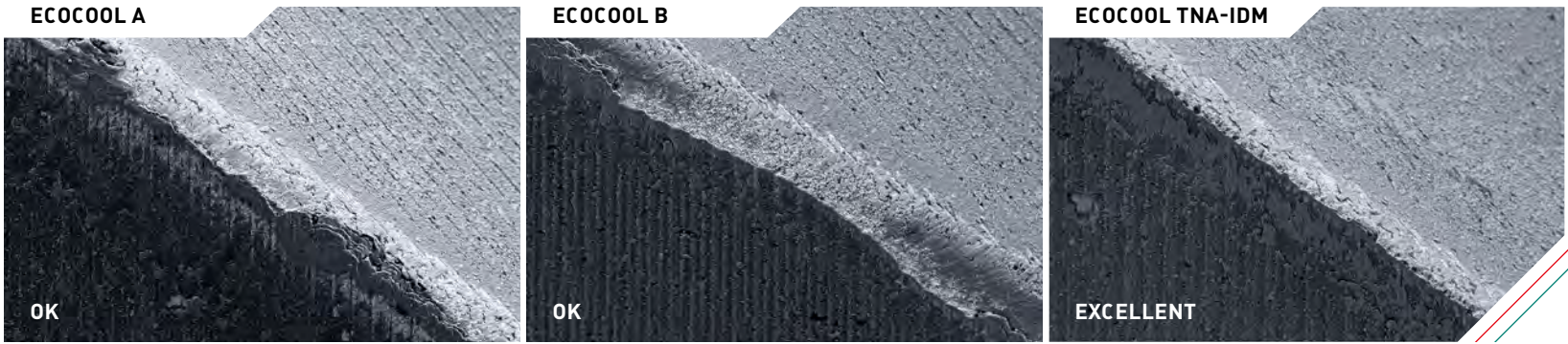
With magnification of the cutting edges under an optical microscope, ECOCOOOL TNA-IDM shows homogenous wear without fracturing of the cutting edges.
