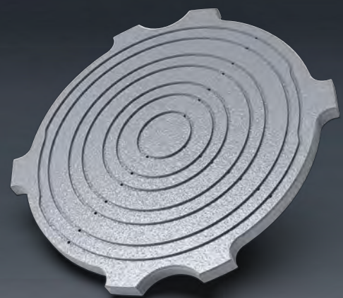
WAFER CHUCK Dimensions: \varnothing 300 \times 10 mm Material: Silicon carbide ULTRASONIC 60 eVo
